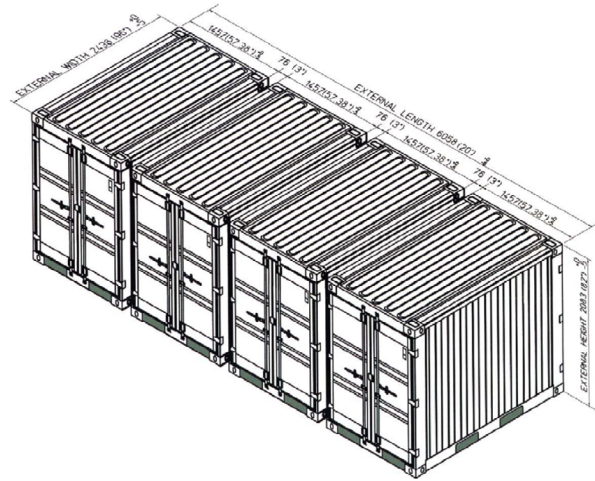
(4) Quadcon Containers coupled together to form one 20' ISO Module
