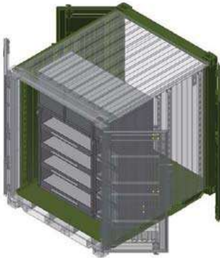
Tricon (Type II) with Modular Cabinet Design Including 2 Base Cabinets with 4 each Roll Out Shelves and 2 Swing-Door Cabinets
