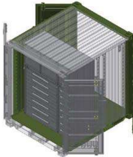
Tricon (Type II) with Modular Cabinet Design Including 14 Drawers and 2 Swing-Door Cabinets
