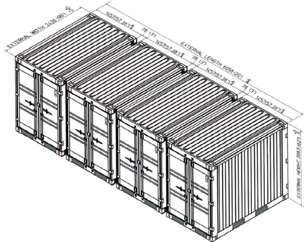
(4) Quadcon Containers coupled together to form one 20' ISO Module
