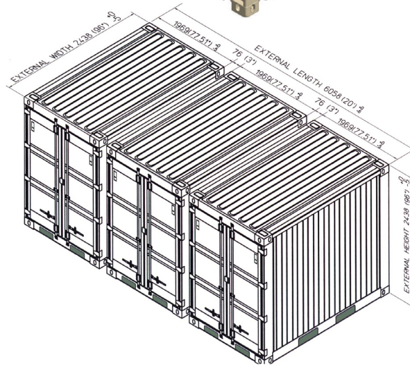
(3) Tricon Containers coupled together to form (1) 20' ISO Module with Fork Pockets 4.5" High x 14.0" Wide Minimum
