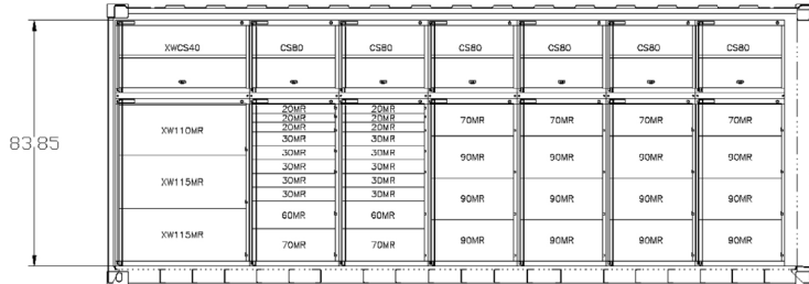
SECTION A INTERIOR CURBSIDE ELEVATION VIEW
