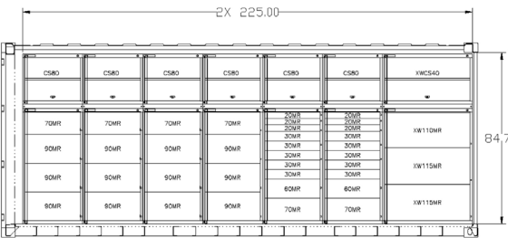
SECTION B INTERIOR ROADSIDE ELEVATION VIEW
