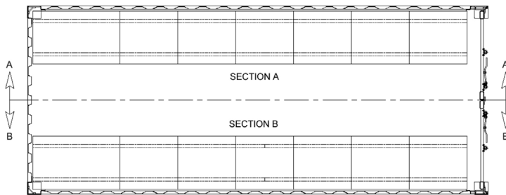
PLAN VIEW, ROOF REMOVED
