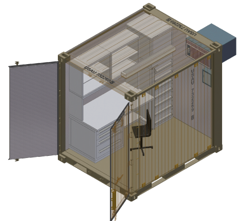
HVAC & Electrical Insert Panel in OFFICE configuration
