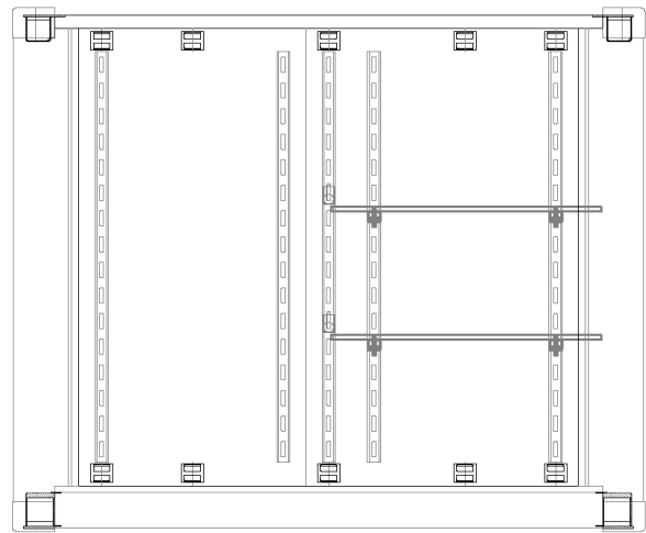
INTERIOR CURB SIDE ELEVATION VIEW
