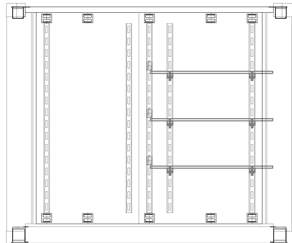
INTERIOR CURB SIDE ELEVATION VIEW
