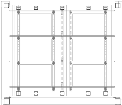
INTERIOR ROAD SIDE ELEVATION VIEW
