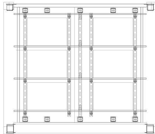
INTERIOR CURB SIDE ELEVATION VIEW
