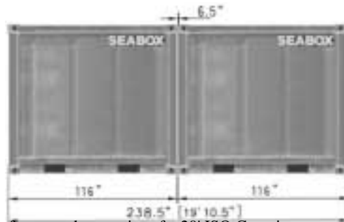
Conforms to the exterior of a 20' ISO Container
