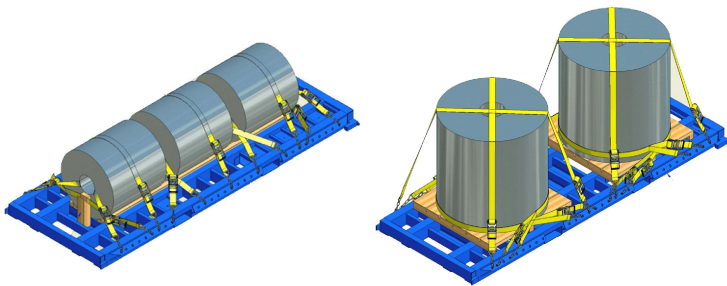
SAMPLE LOADS
