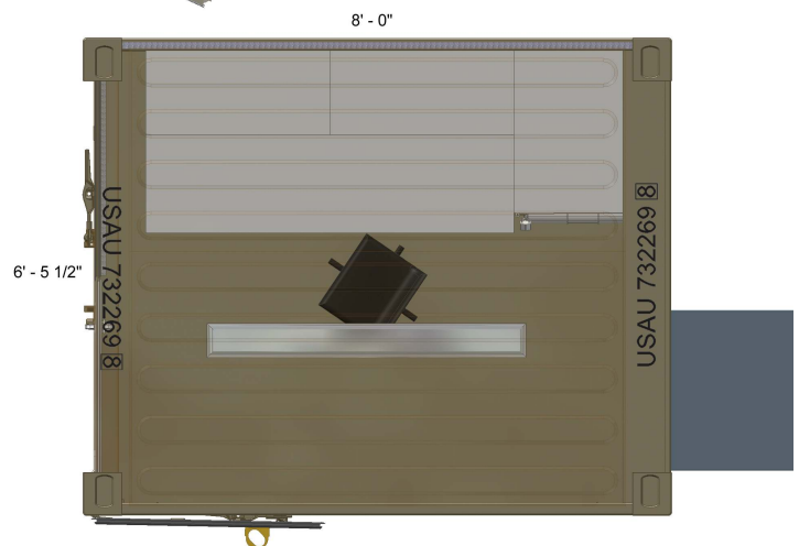
PLAN VIEW; ROOF REMOVED
