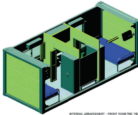
INTERNAL ARRANGEMENT - FRONT ISOMETRIC VIEW
