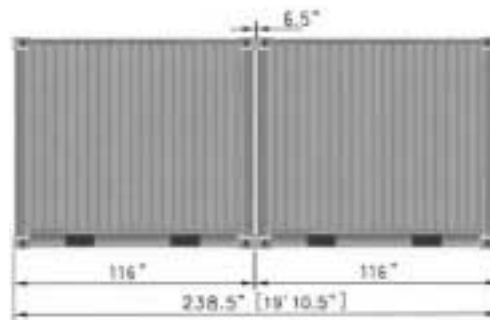
Conforms to the exterior of a 20' ISO Container Designed to fit on a standard 23' Container Chassis Trailer
