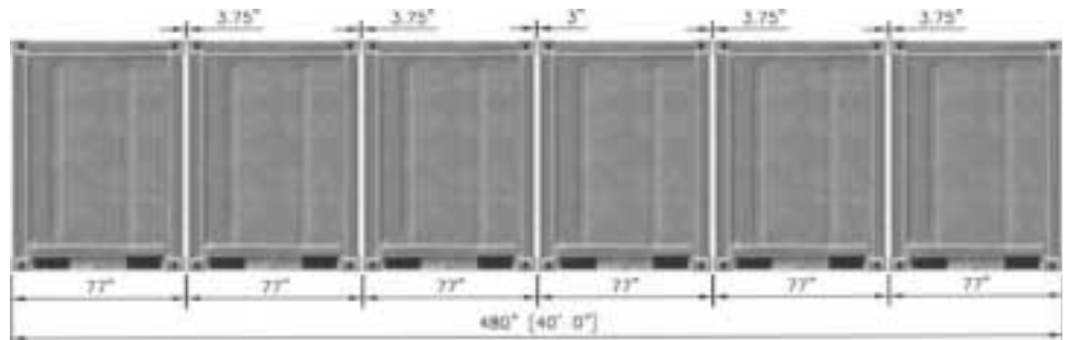
Designed to fit on a standard 40' Straight Frame Container Chassis Trailer
