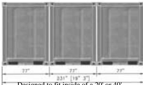
Designed to fit inside of a 20' or 40' (8' 6") ISO Container
