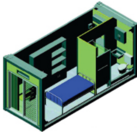
INTERNAL ARRANGEMENT - FRONT ISOMETRIC VIEW
